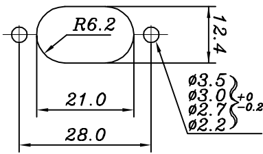
PANEL CUT-OUT
